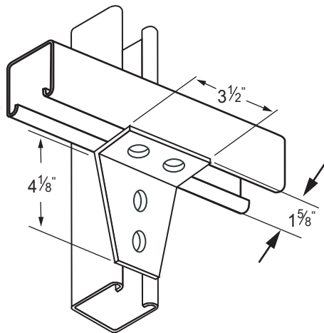
D118 Four Hole Joint Connector
