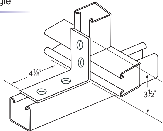
D103 Three Hole Corner Connector Wt.56#/C
