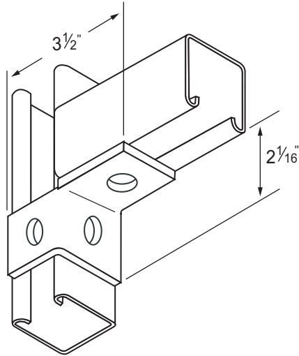
B267L - B267R Three Hole Single Angle Connector (right angle shown)
