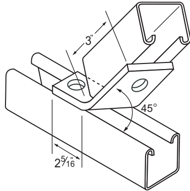
D154 Two Hole Open 45° Angle
